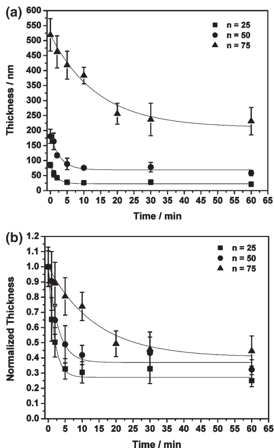
Figure 4. (a) Absolute and (b) normalized thickness of \text{Chi}(\text{PB}/\text{Chi})_5(\text{PB}/\text{GS})_n films over time at an applied potential of +1.25 V vs Ag/AgCl in a PBS, pH 7.4 electrolyte. The thickest films dissolve more slowly, and all film thicknesses plateau to approximately 25–45% of initial thickness. The lines represent the best fit to a first order exponential decay model. Error bars represent \pm 1 standard deviation in measured thickness values at n = 5 –10 locations on each film.
