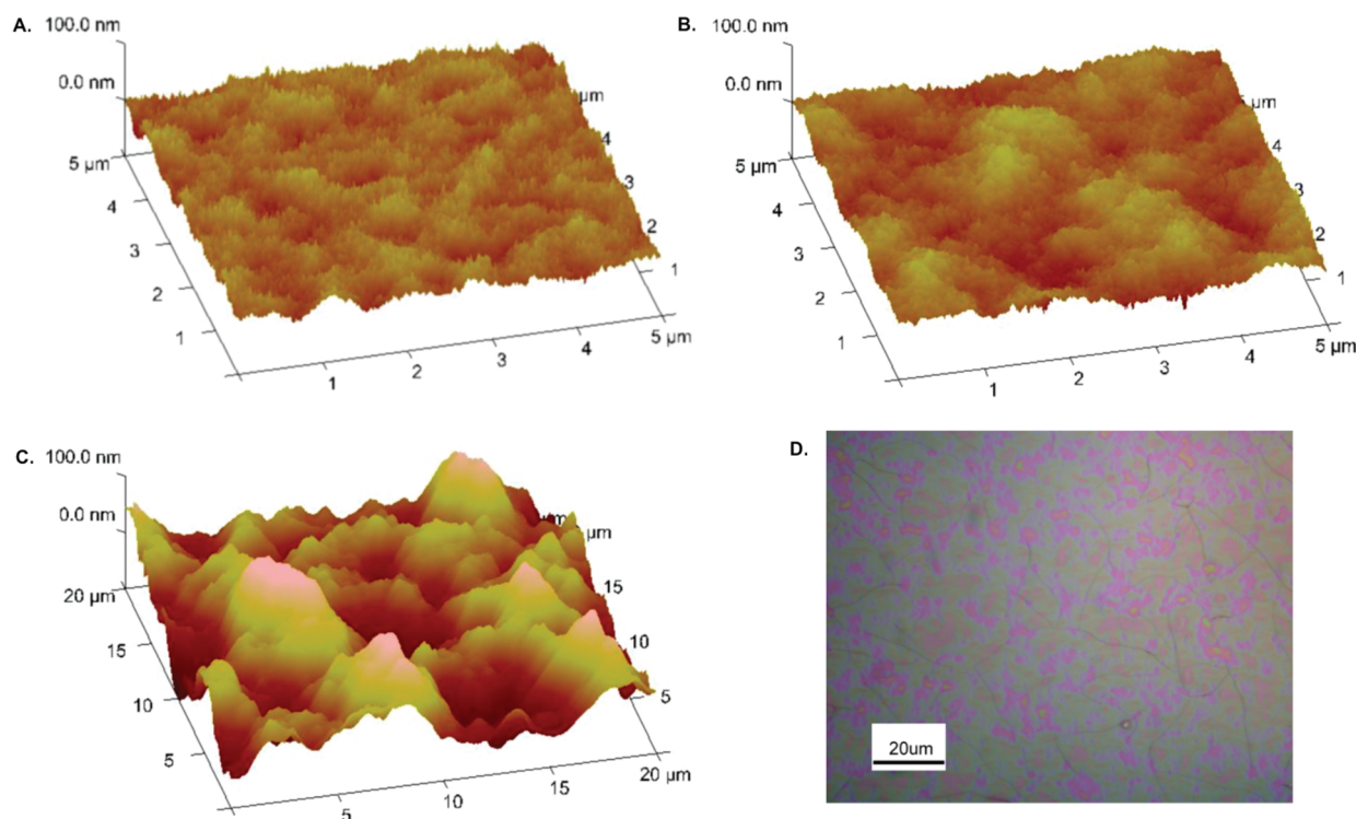
Figure 2. Atomic force microscopy 3D height images of (A) n = 25 , (B) n = 50 , and (C) n = 75 bilayer films and (D) an optical micrograph of an n = 75 film. Film surface roughness increases and clusters form on the film surface with the deposition of an increasing number of bilayers.
