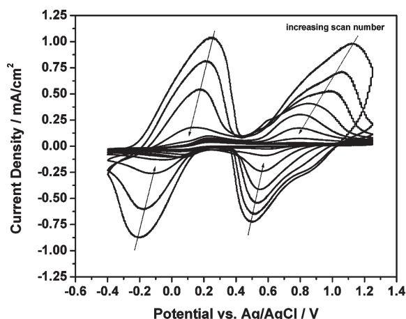
Figure 3. Cyclic voltammograms of a \text{Chi}(\text{PB}/\text{Chi})_5(\text{PB}/\text{GS})_{25} film subjected to multiple cycles at a scan rate of 50 mV/s in a PBS, pH 7.4 electrolyte. A decrease in peak height (and peak area) with subsequent scans reveals a loss of the electroactive Prussian Blue from the film.
